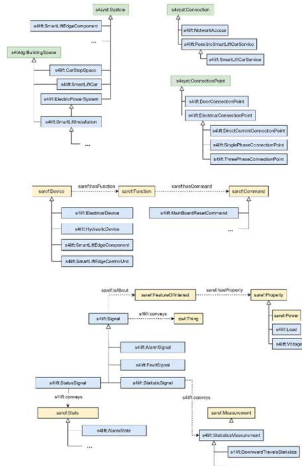
Figure B-1: Conceptual model containing the new concepts defined through the use case analysis and their relationships
